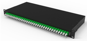
1RU panel, 1X16 split ratio, 4 splitters, LC/APC connectors
